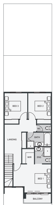
UPPER FLOOR PLAN
